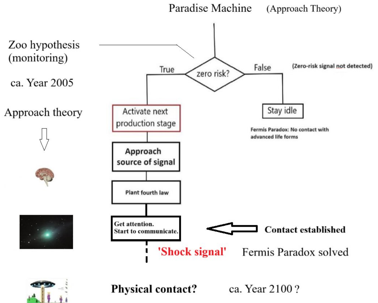
Figure 7. Modified figure 19 from the 2024 paper shows a suggested pre-stored protocol that is activated if the unique signal for zero-risk is detected by Fermi life-forms, transmitted from another life form anywhere in the universe.
